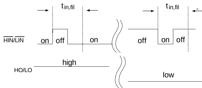
Figure 5.5 Input Filter Function
